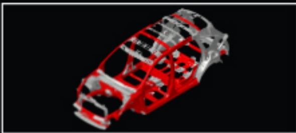
G-CON + ACE™ with Side Impact Beam
